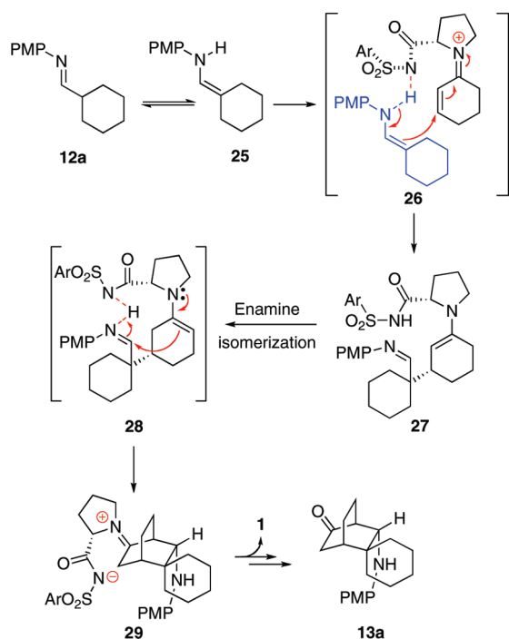
SCHEME 4. Possible Mechanistic Hypothesis for Formation of Amine 13a
