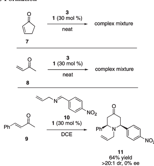
SCHEME 1. Exploration of Alternate Enone Systems in the Bicycle Formation
