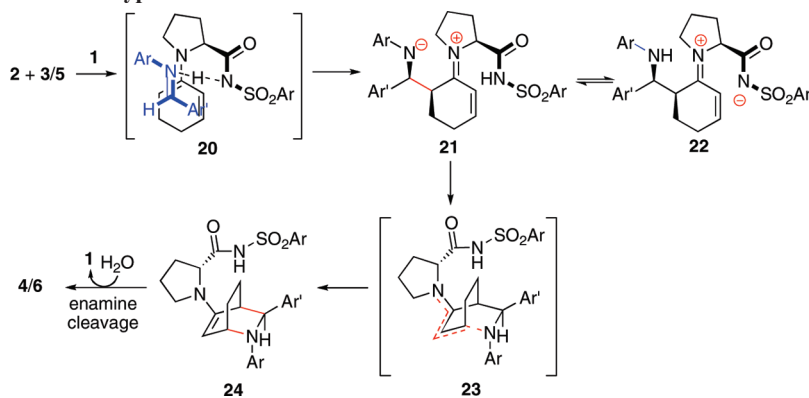
SCHEME 3. Possible Mechanistic Hypothesis for Formation of Amines 4 and 6
